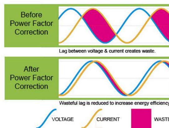
Figure 30. Effect from using a Power Factor Correction Device
